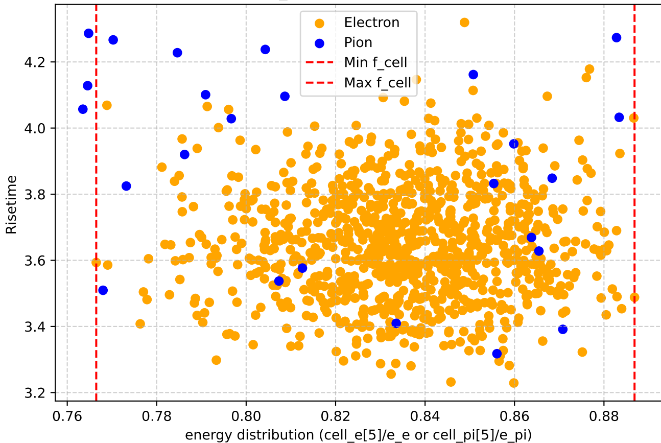
Scatter plot of f_{\text{cell}} vs risetime for energy 5.0GeV
